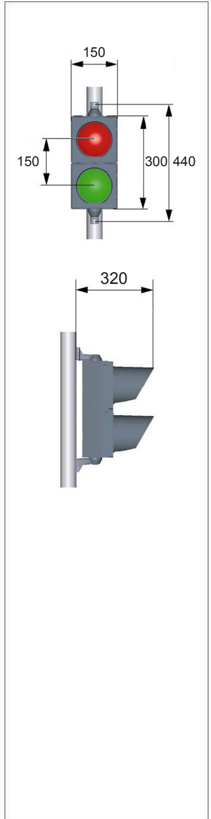
dimension drawing
